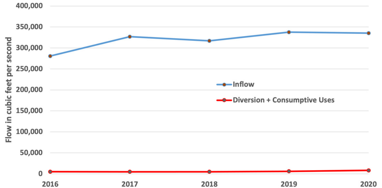
Figure 21. Cumulative hydrologic effects on flows for Lake Ontario, 2016-2020.
